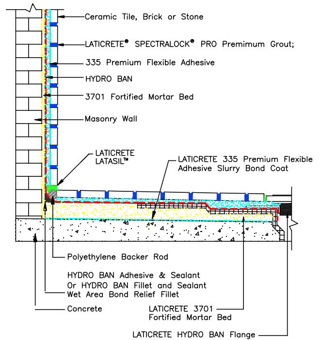
Detail 4 - HYDRO BAN Flange
