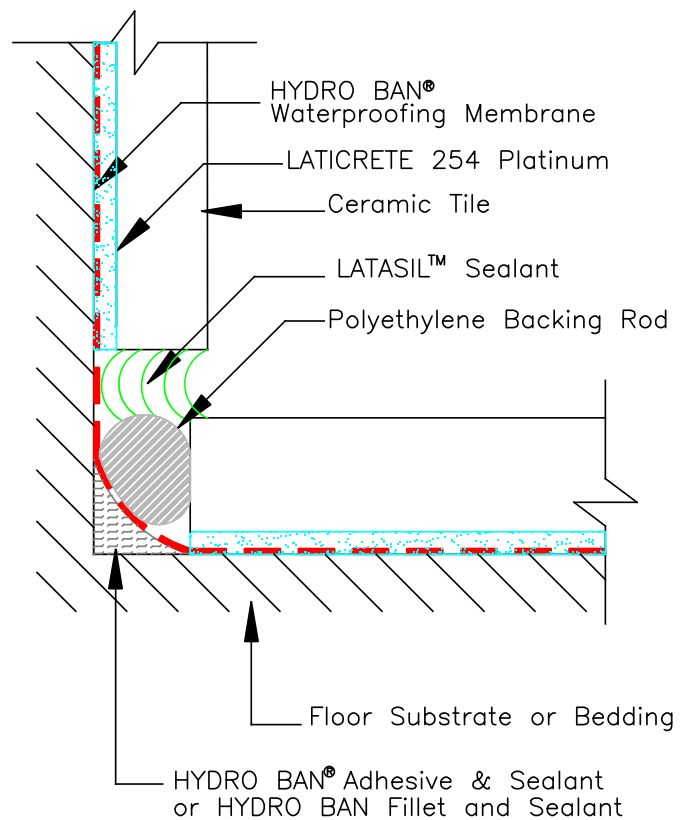
Detail 2 - Typical Thin Bed Installation
